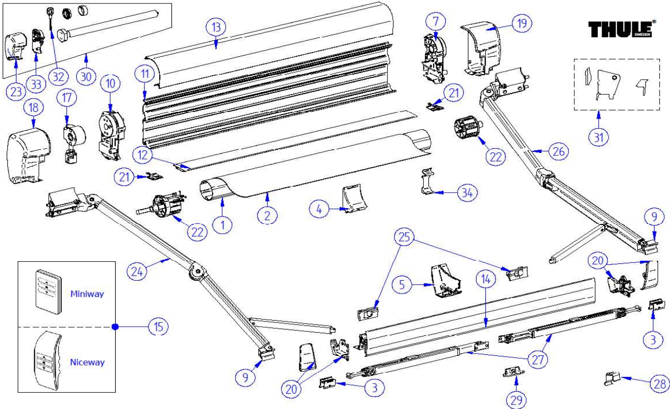
THULE Omnistor 8000
